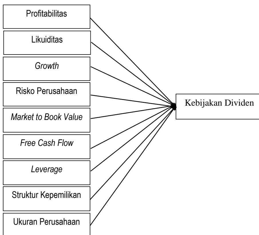
Gambar 1 Model Penelitian
